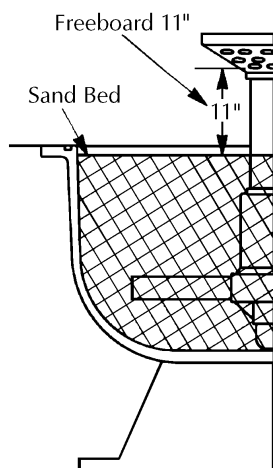
Figure 2 - Freeboard measurement
